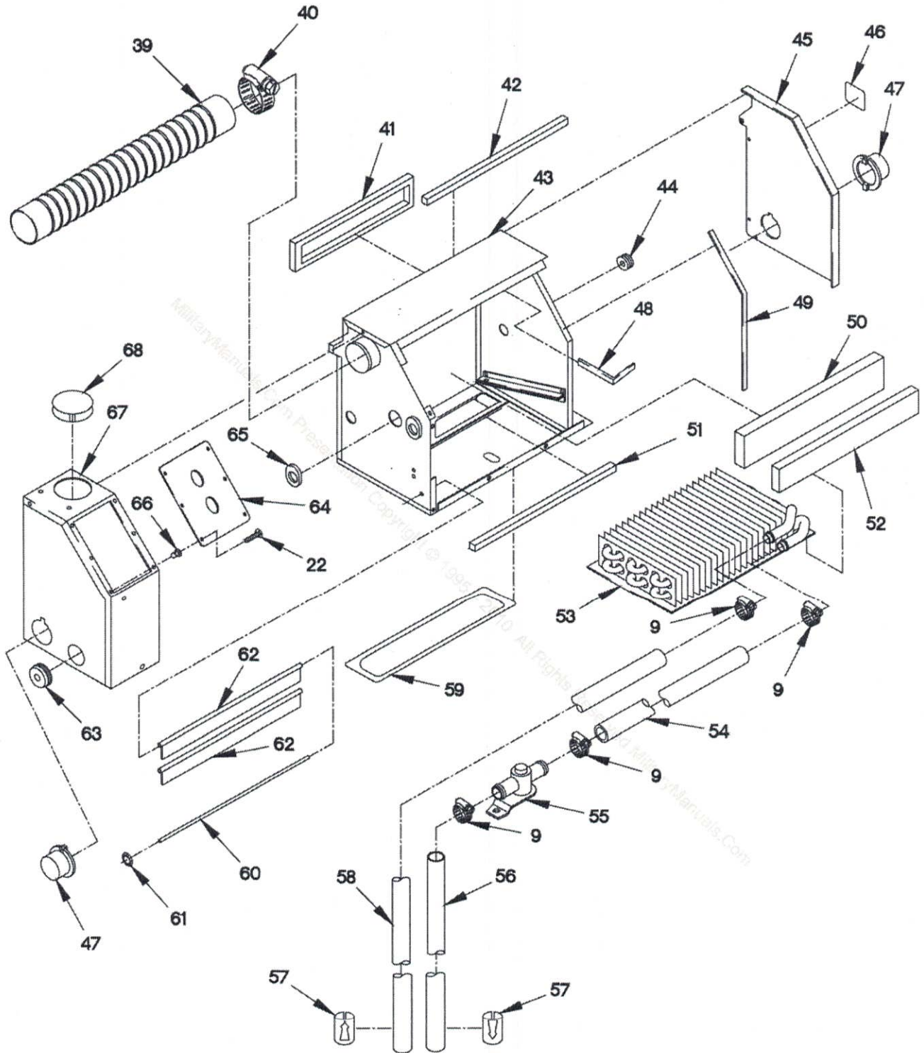
FIGURE 251. PERSONNEL HEATER ASSEMBLY (SHEET 3 OF 3)
